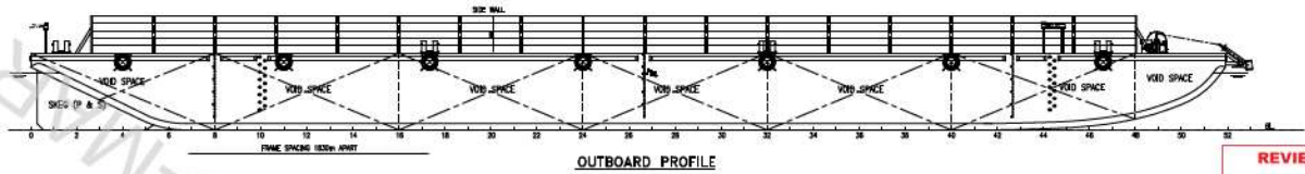
OUTBOARD PROFILE
